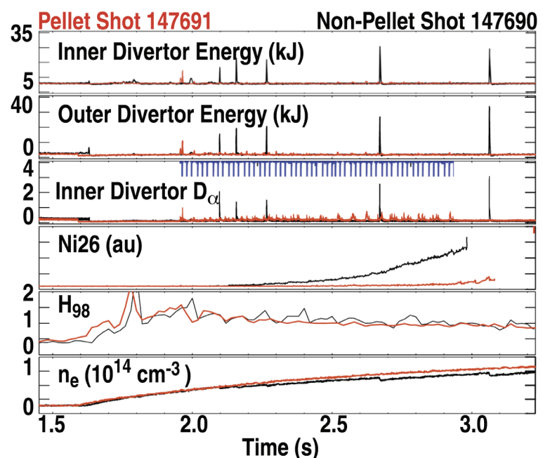
Fig. 2. Comparison of 60 Hz pellet case (red) and no-pellet plasma with 5 Hz ELMs (black). Divertor deposited energies and divertor particle flux are shown with nominal pellet times by blue tick marks. Central Ni emission, normalized energy confinement H_{98} , and electron density are shown.
