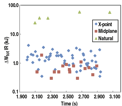
Fig. 3. Energy deposited (log scale) in the divertor from the IR camera data for each ELM in the discharges shown in Fig. 2. The natural ELMs are from the non-pellet comparison discharge.
