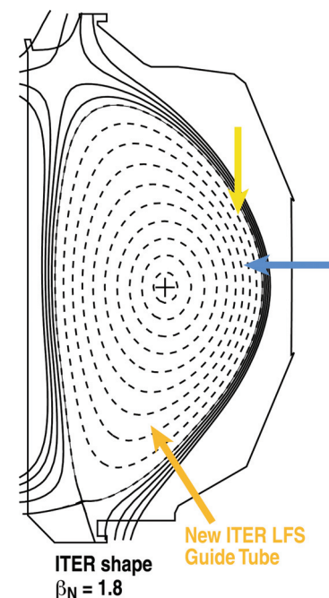
Fig.1. Pellet injection geometry used for EM pacing studies on DIII-D. The lower trajectory is similar to the planned ITER low field side injection line for pellet ELM pacing.
