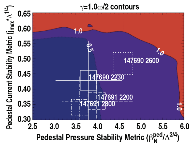
Fig. 4. Normalized shear plotted against normalized pressure for the pedestal location on these pellet (147691) and non-pellet (147690) comparison discharges in Fig. 2. ELITE calculation of the boundary for peeling and ballooning stability is shown for this plasma configuration.
