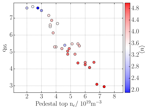
Figure 1: Averaged toroidal mode number dependence on density and q_{95} , where the blue to red color range stands for low to high n .
