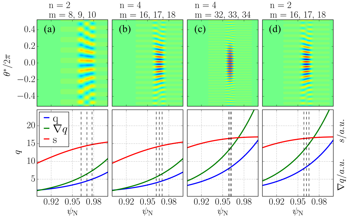
Figure 2: (Top) Artificial mode structures in the \theta^*/\psi_N plane for (bottom) two different q , \nabla q and s profiles: (a, b) weak shear with q_{95} = 3.2 and (c, d) stronger shear with q_{95} = 7.0 .
