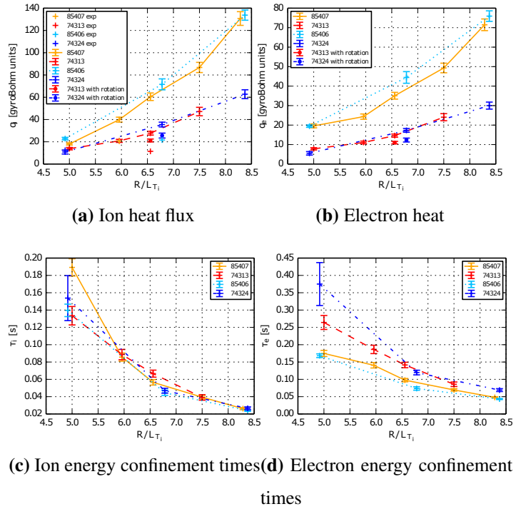
Figure 2: Nonlinear R/L_{T_i} scans, electron and ion heat flux and energy confinement times
