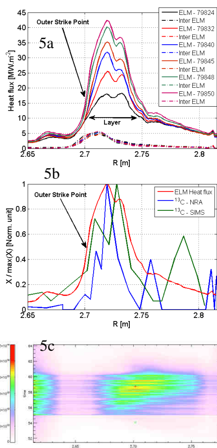
Fig.5: a. ELM and inter ELM heat profiles for 6 different discharges with 13 CH 4 injection. The heat flux apparent increase is attributed to the growth of a layer revealed by post-mortem analysis (b). C. In situ spectroscopy – CH A-X emission.
