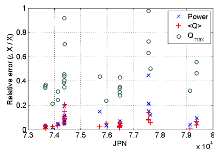
Fig.6: Influence of thermal properties modification on the power, Q_{\text{max}} and \langle Q \rangle , respectively maximum and average heat flux measured on the target.
