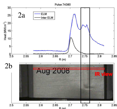
Fig.2: (a)ELM heat flux profile exhibits a peak at 2.75m that can be associated with an alteration of the tile's surface seen on the visible image (b).
