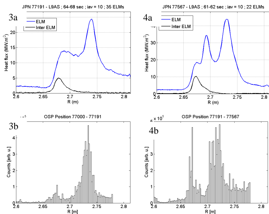
Fig.3: (a) ELM and inter ELM heat profiles on outer target. A peak two times higher than the OSP is observed at 2.74m. (b) Location of the OSP on the outer target for pulses from JPN 77000 to 77191.
