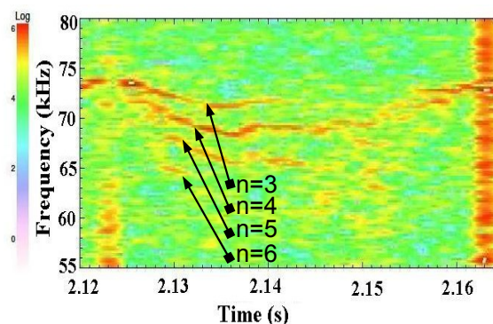
Figure 1: Mode activity during sawtooth cycle.
