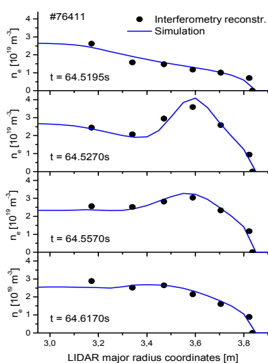
Figure 3 – Simulated density evolution for a pellet ( r_p = 1.6 mm, V_p = 160 ms -1 ) injected from the LFS into a JET L-mode target plasma assuming increased edge particle transport (5x compared to Bohm/gyroBohm level) after injection; the data is compared with profile reconstructions from interferometry data.
