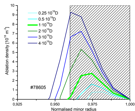
Figure 5 – Pellet ablation profiles for small pellets injected from the LFS into a JET H-mode plasma; pellets with a mass of > 10^{19} D seem to reliably trigger ELMs [2]. The shaded area indicates the ETB zone.
