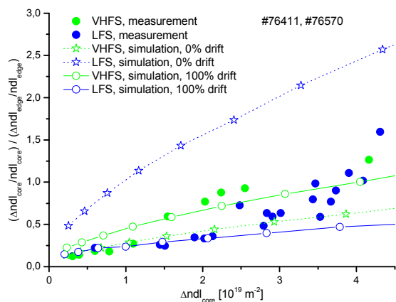
Figure 1 – Ratio between the relative increase of line-integrated plasma core and edge densities measured along the JET interferometry lines of sight versus the increase in line-integrated core density after pellet injection.
