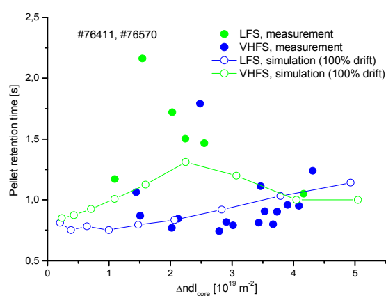
Figure 2 – Pellet particle retention time measured as exponential decay time of the line-integrated plasma core density signal after pellet injection versus the pellet-caused increase in line-integrated core density.
