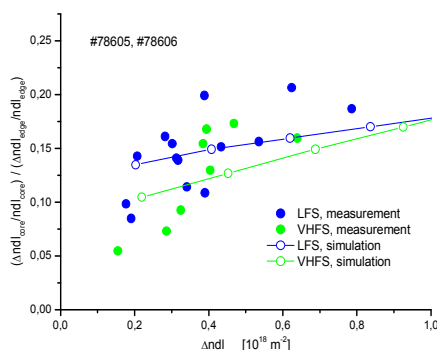
Figure 4 – Ratio between the relative increase of line-integrated plasma core and edge densities measured along the JET interferometry lines of sight versus the increase in line-integrated core density after pellet injection. According to the simulation results, the upper mass limit is \approx 4 \cdot 10^{19} D.
